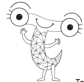
Tau
