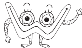
W boson
